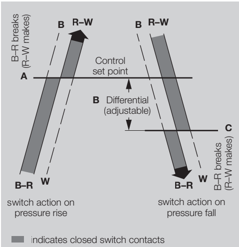
Operation of switch on pressure rise and fall
